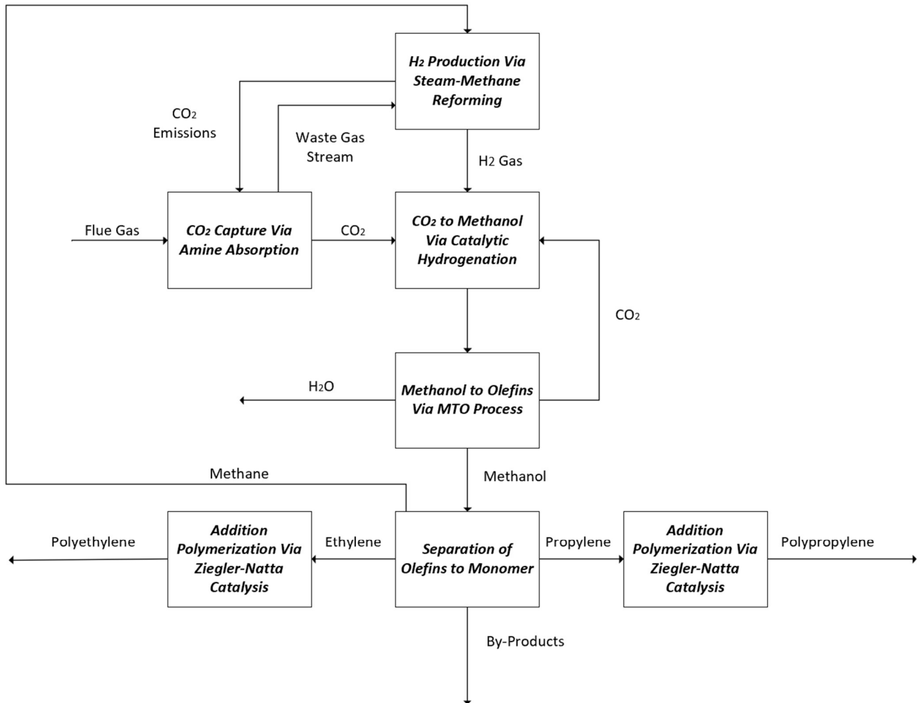
Figure 13: Block Flow Diagram of the Proposed Ideal Process
