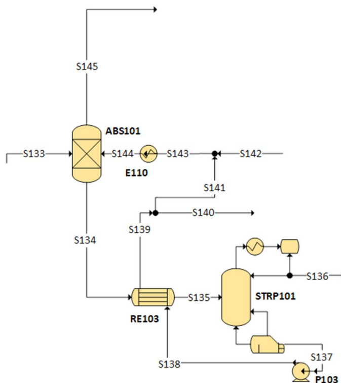
Figure 19: Absorber Section for Methanol to Olefins Process
