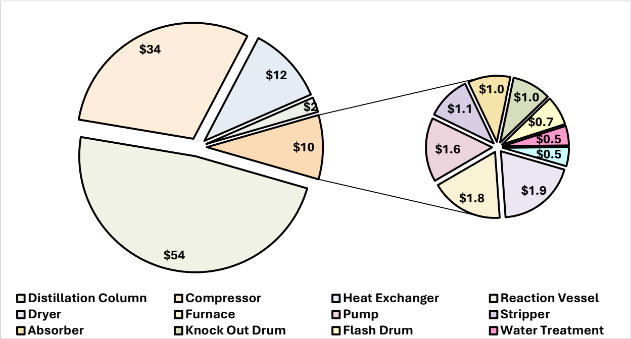
Figure 23: ISBL Cost Split into Equipment Type
