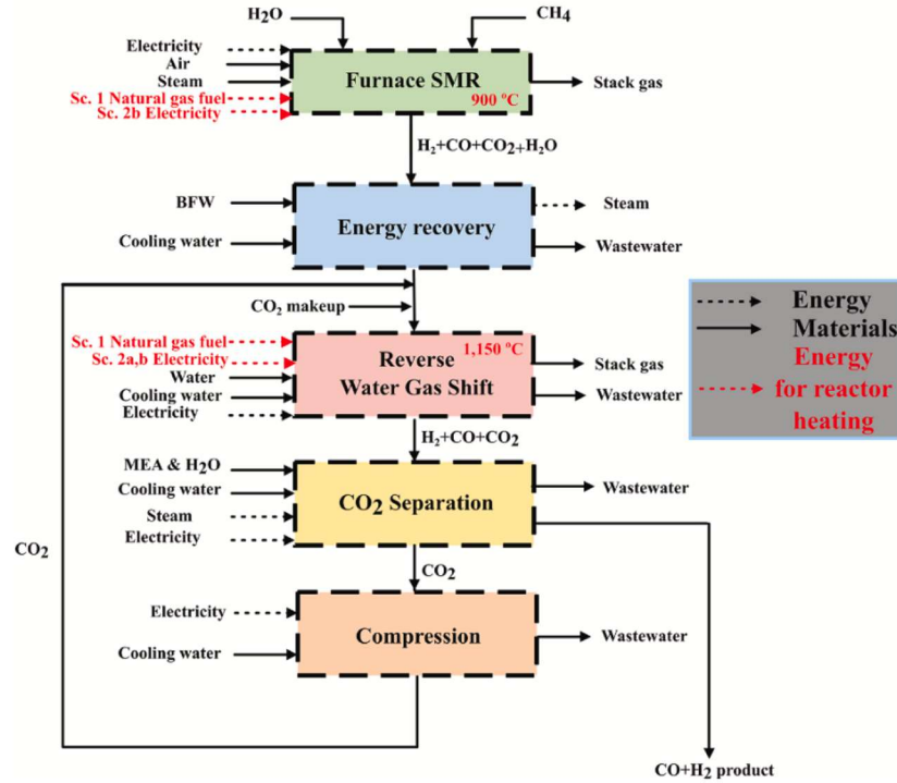
Figure 9. SMR + RWGS for CO 2 to Syngas (Cao, 2022).
