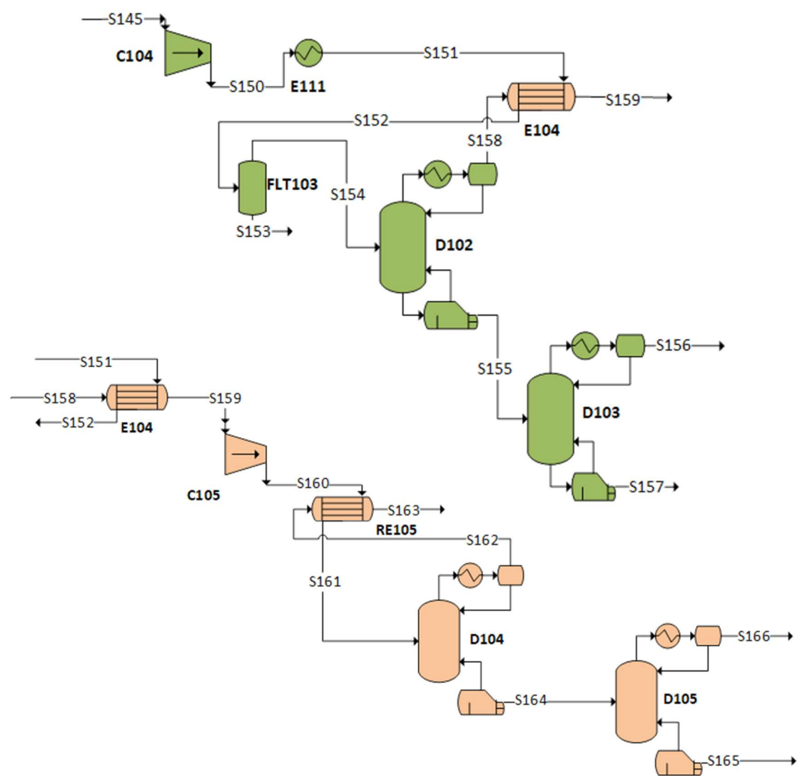
Figure 20: Purification Section for Methanol to Olefins Process
