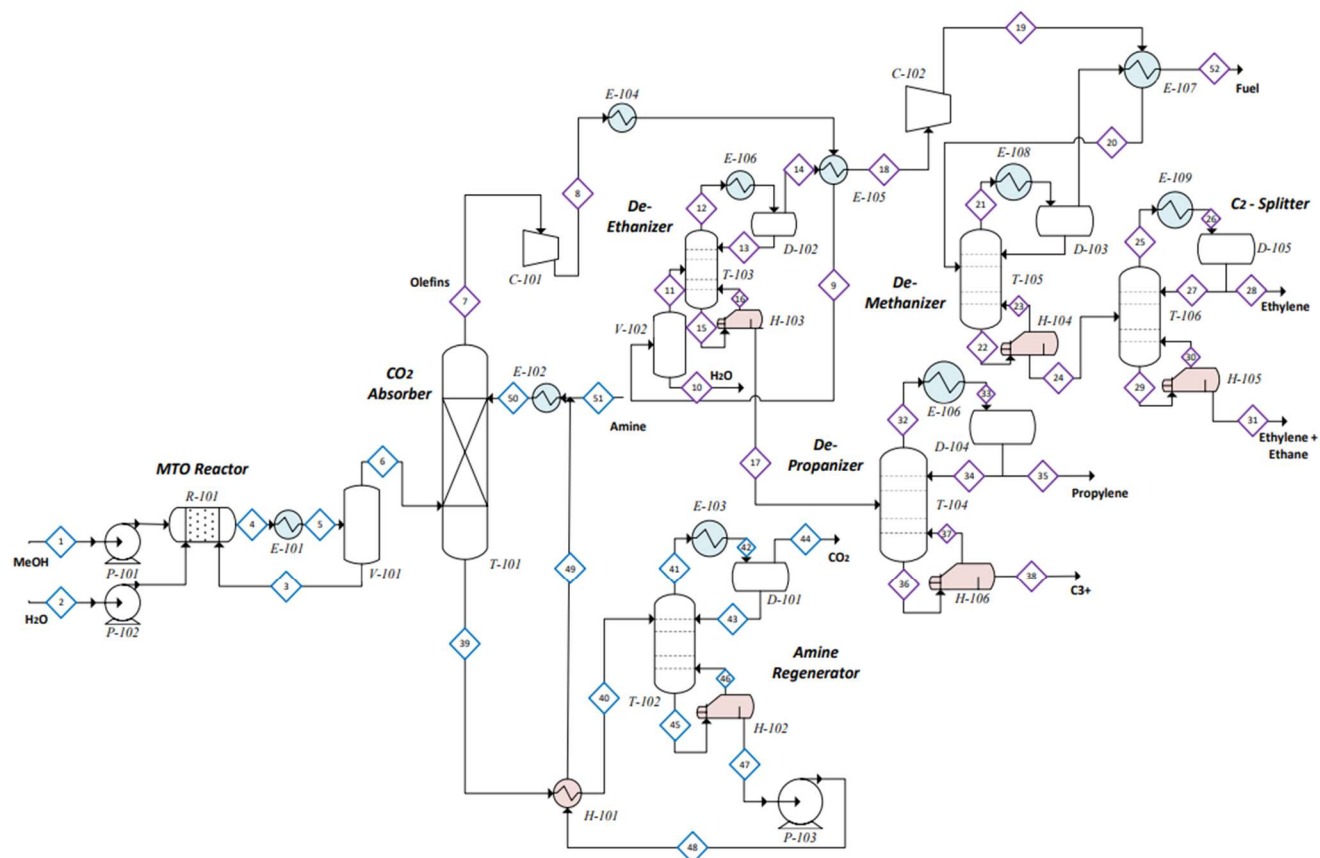
Figure 15: Methanol to Monomer Process Flow Diagram
