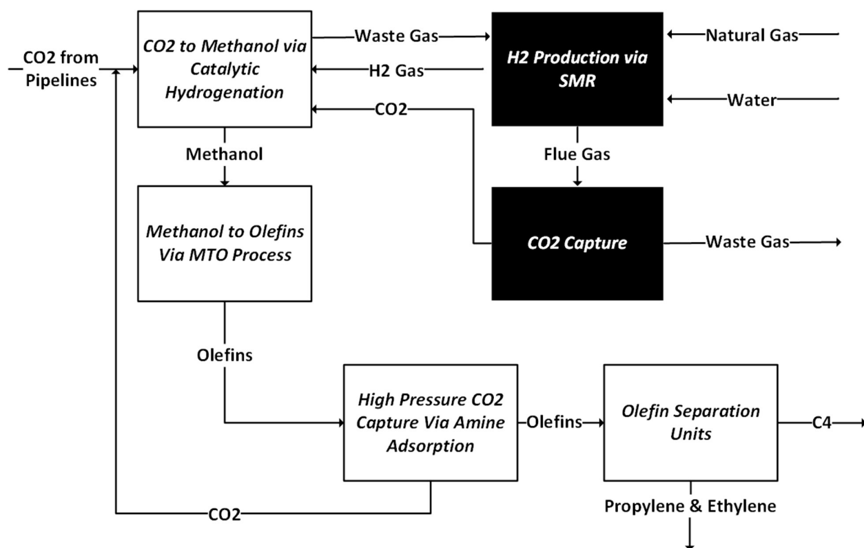
Figure 12: BFD of the Current Process
