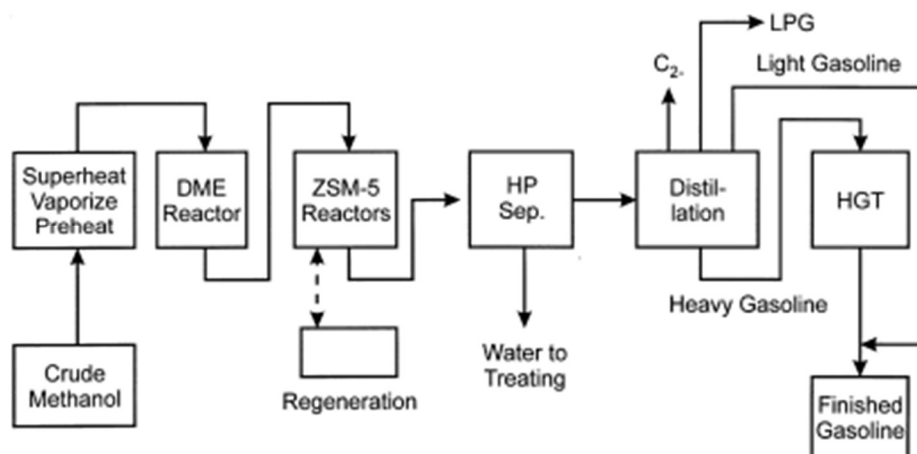
Figure 7: MTG Block Flow Diagram (Keil,1999).
