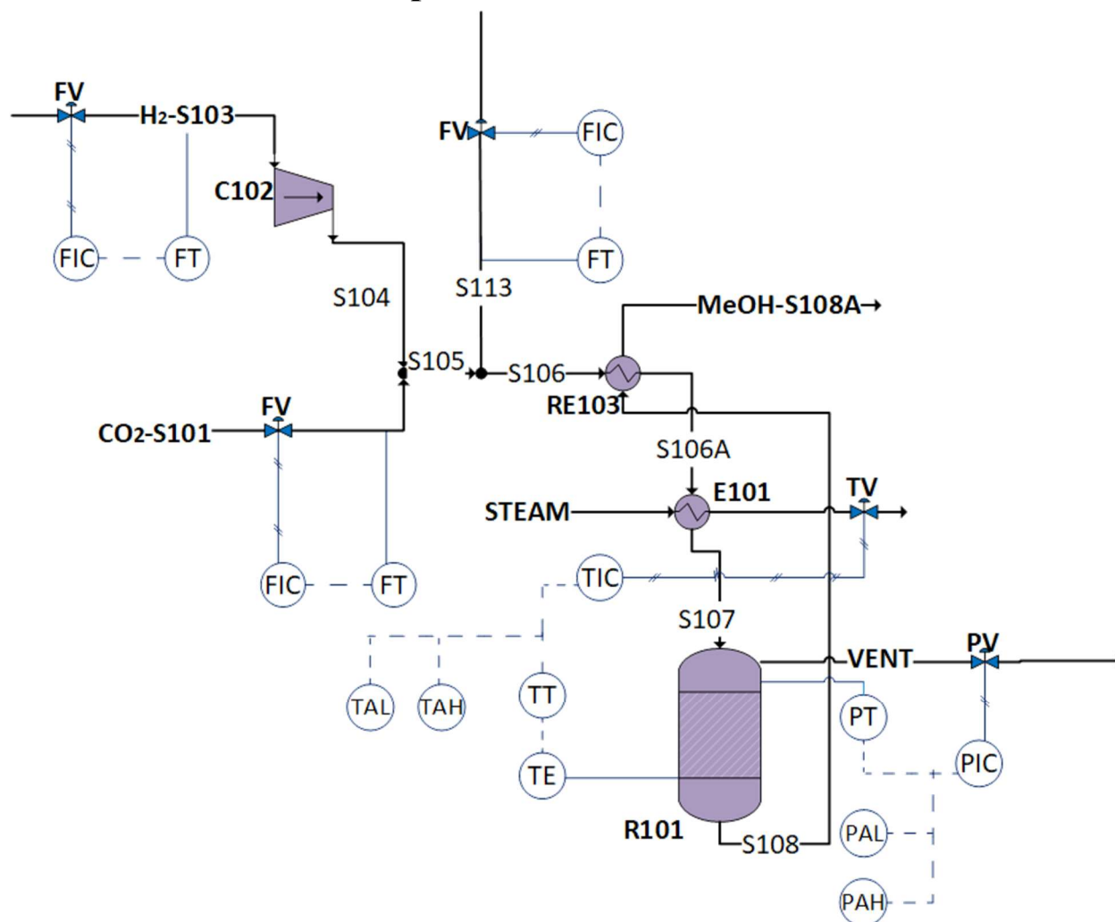
Figure 10: Process Control Loop over R-101
