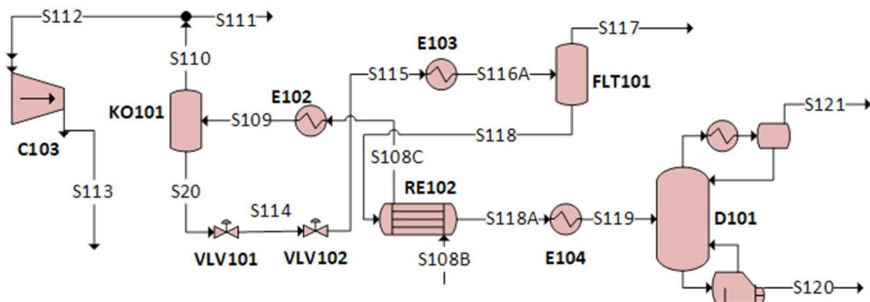
Figure 17: Purification Section for CO 2 to Methanol Process
