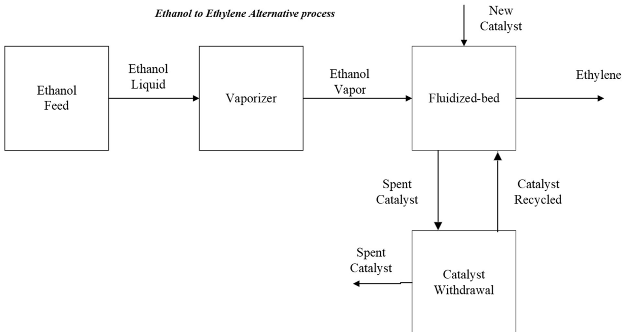
Figure 8: Ethanol to Ethylene Block Flow Diagram
