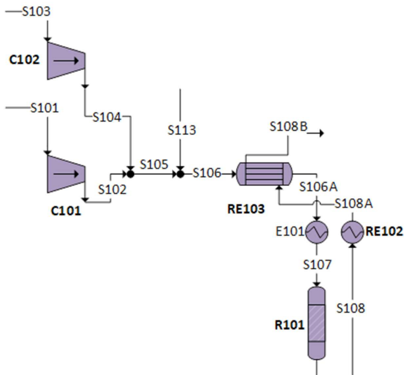
Figure 16: Reaction Section for CO 2 to Methanol Process
